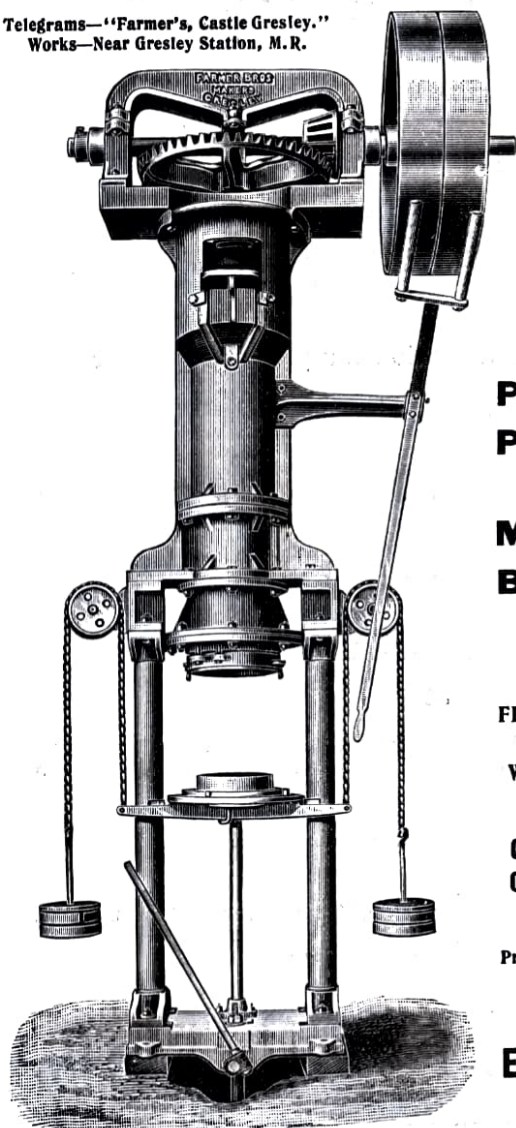
Improved Self-Socketing Pipe Machines in Stock or Progress.
